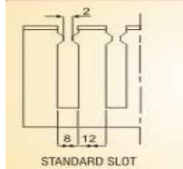
STANDARD SLOTS
