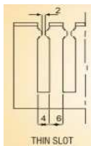
THIN SLOTS
